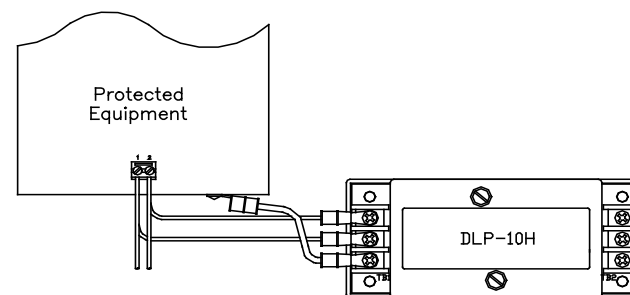
Figure 2 (Parallel wiring diagram for models ending in "V0" only)
